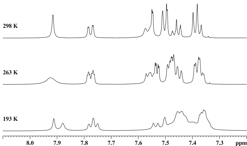
Figure 2. Aromatic region of ^1\text{H} NMR spectra of 7 in \text{CD}_2\text{Cl}_2 at variable temperatures.
