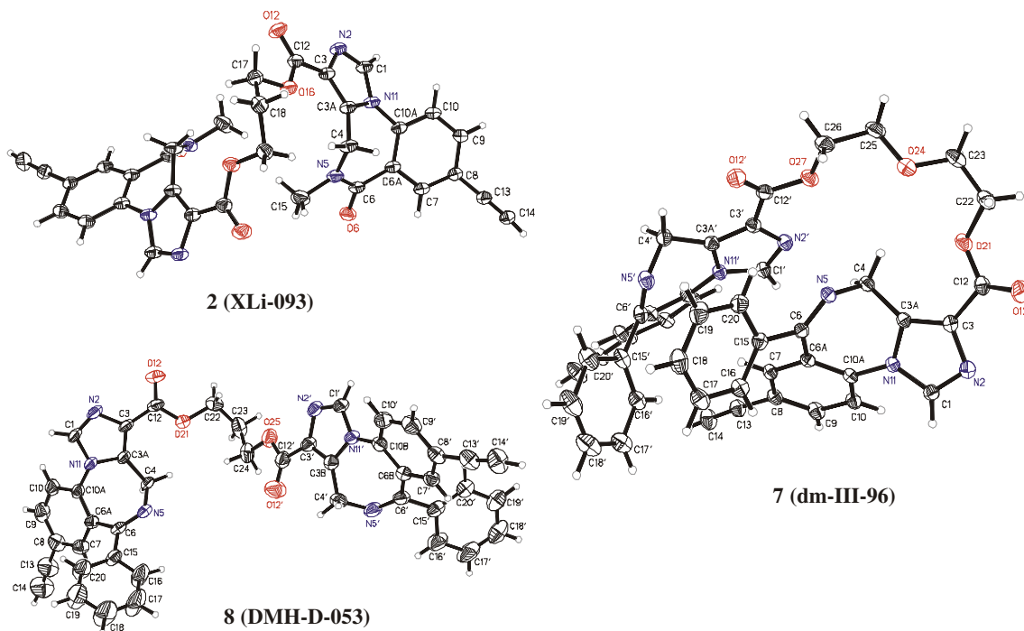
Figure 1. Crystal structure of 2 (left top), 7 (right) and 8 (left bottom).
