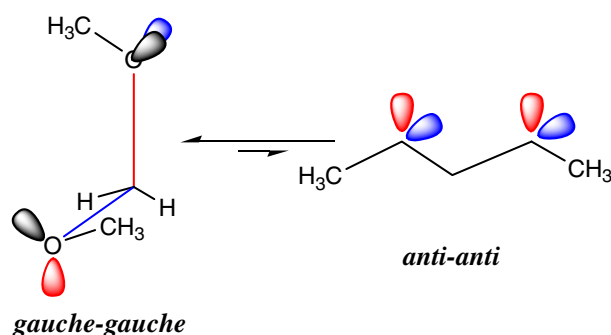
Figure 9. The conformations for dimethoxymethane.
