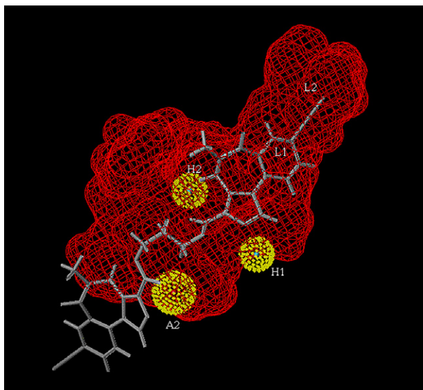
Figure 7. Bivalent ligand 2 (Xli093) aligned in the included volume of the pharmacophore/receptor model for the \alpha 5\beta 3\gamma 2 subtype.
