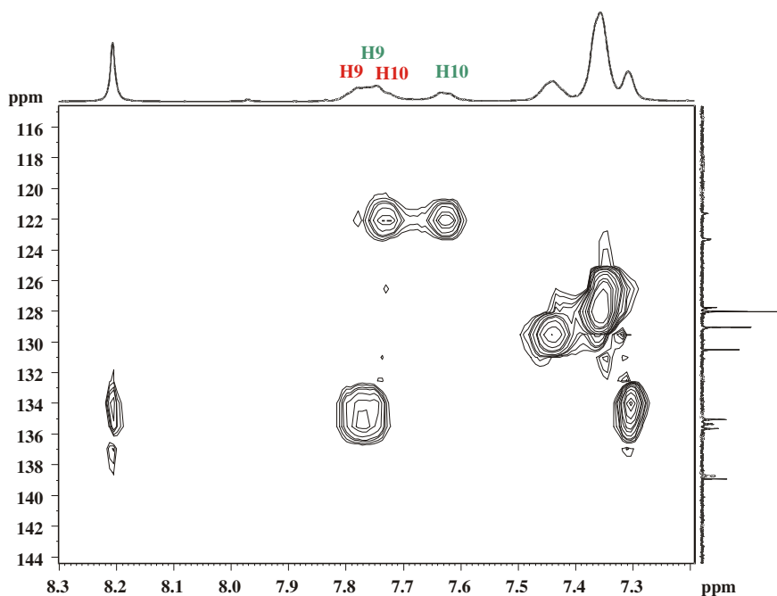
Figure 6. Partial HSQC spectrum of 7 in MeOH- d_4 at 298 K.
