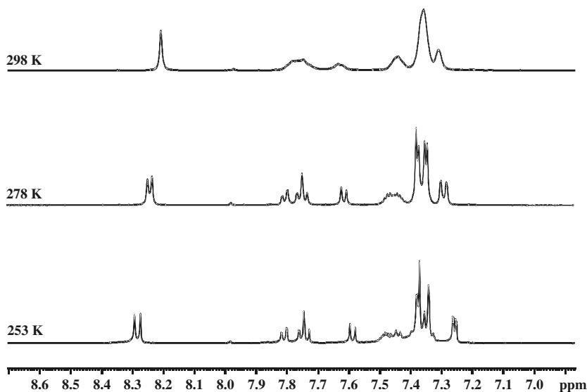
Figure 5. Aromatic region of proton spectra of 7 in MeOH- d_4 at different temperatures.
