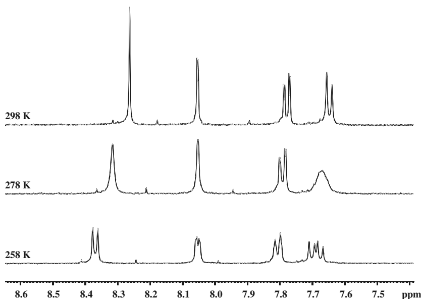
Figure 4. Aromatic region of ^1\text{H} NMR spectra of 2 in \text{MeOH-}d_4 at different temperatures.
