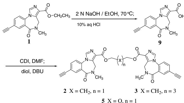
Scheme 1. Synthesis of bivalent analogs of Xli093.
