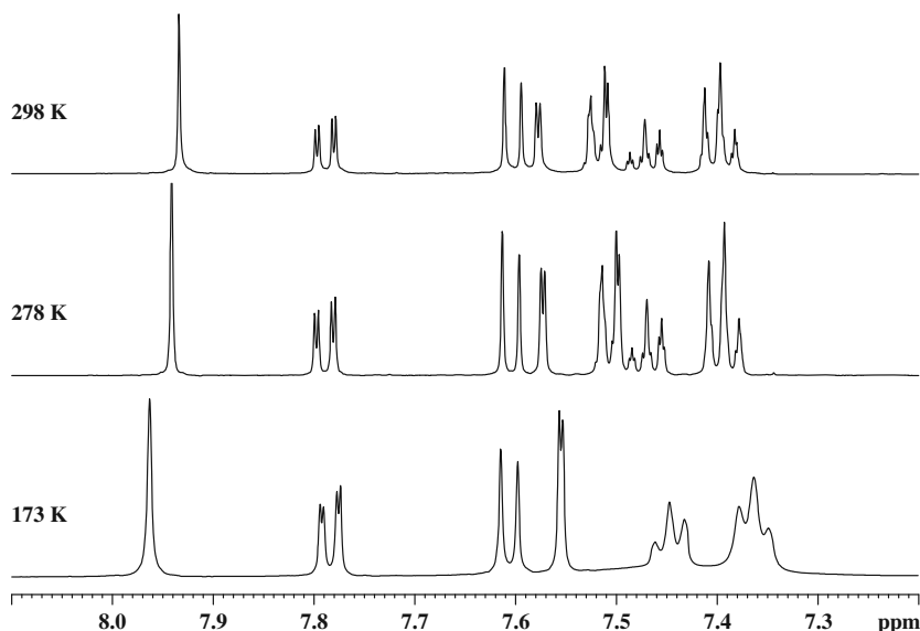
Figure 3. Aromatic region of ^1\text{H} NMR spectra of 6 in \text{CD}_2\text{Cl}_2 at different temperatures.
